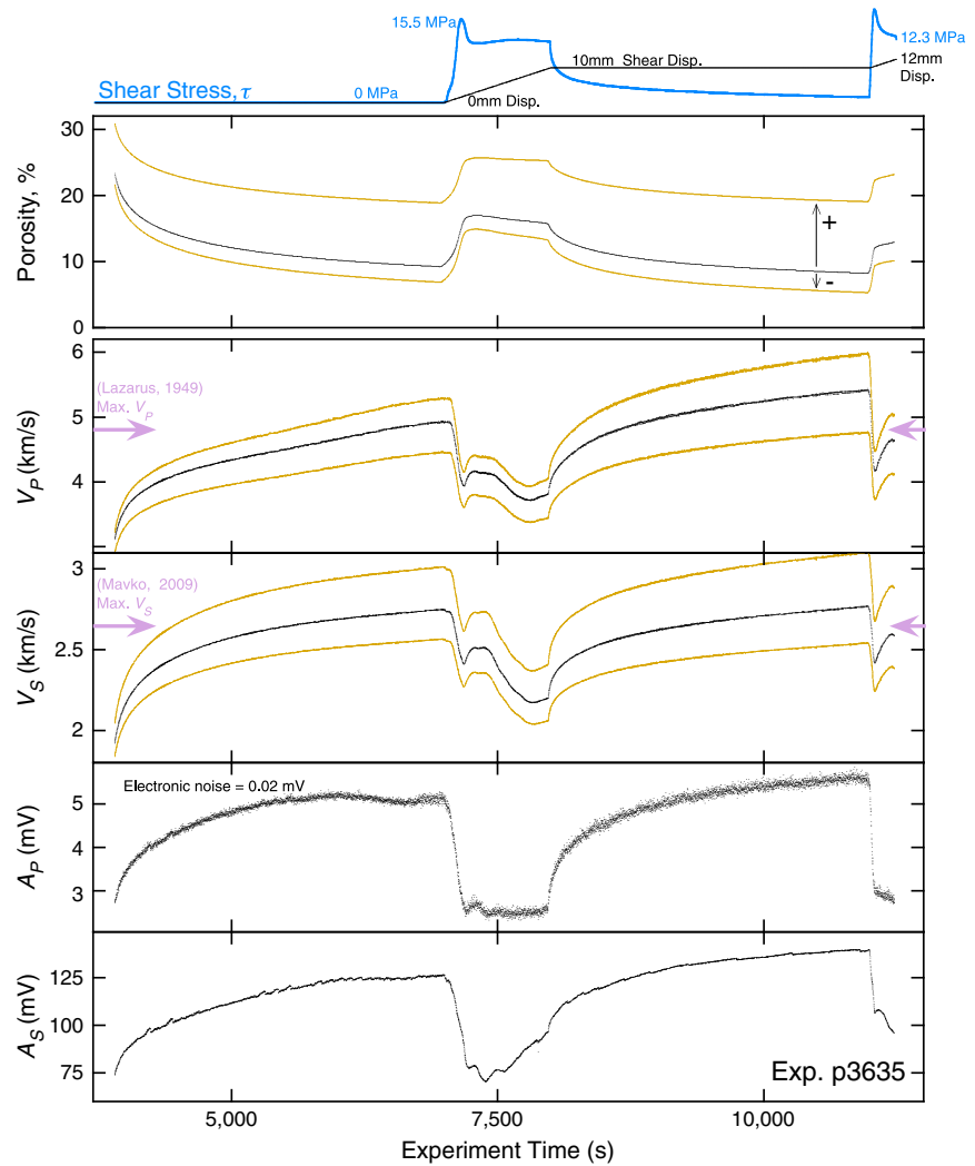
Figure 5. Porosity, velocity, and amplitude changes and uncertainty in an experiment with shear. Porosity decreased and V_P , V_S , A_P and A_S increased during hold periods, similar to Figure 4, and these trends reversed during shear periods. Velocities and amplitudes typically relate inversely with \phi changes.
