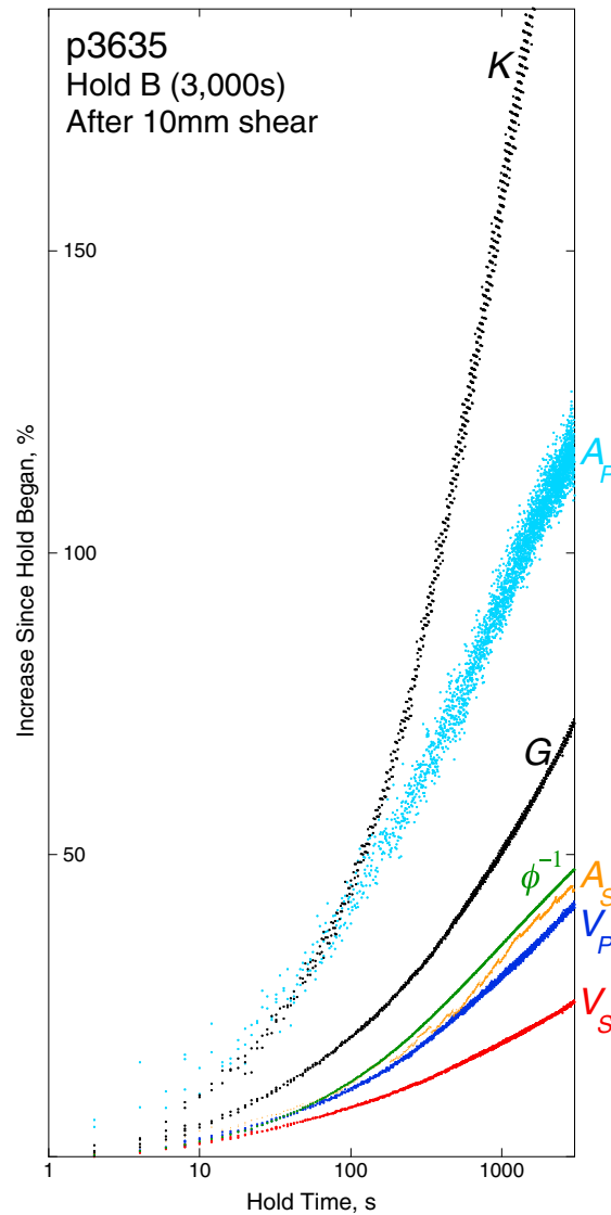
Figure 11. During holds, elastic wave speeds and amplitudes increase with log time along with \phi decrease. A_P changes were strongest, increasing by 55% per decade. Initial changes ( < \sim 300 s) in \phi , velocities, and amplitudes were limited, perhaps owing to a “cutoff time” for dominant pressure solution [Niemeijer et al., 2008].
