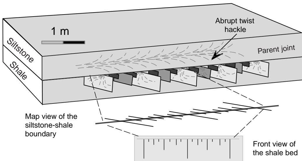
Figure 2. Schematic of an abrupt twist hackle. These fringe cracks can propagate downward or upward from a siltstone bed into adjacent beds. They have a characteristic sequence of large and small cracks, indicative of suppressed growth where crack stress shadows limit the growth of some cracks.
