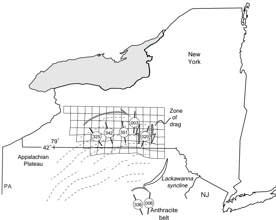
Figure 17. Deformed-state grid given by the displacement field determined from finite strain as indicated by deformed crinoid columnals and cleavage (adapted from Geiser, 1988). Dashed lines are traces of the fold axes. The samples with numbers indicate the trends of joint sets from the Appalachian Plateau (this study) and data on the orientation of the Alleghanian stress field in the anthracite belt of Pennsylvania (Gray and Mitra, 1993).
