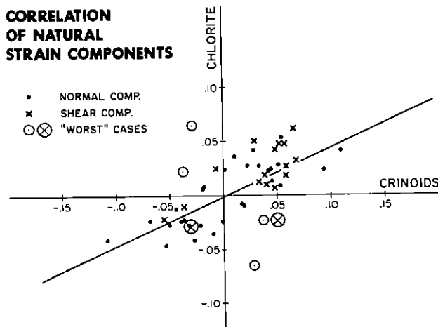
Fig. 6. Correlation of components of natural strain from preferred orientation of chlorite, p_{n_{ij}} (ordinate), with those from crinoid columnar shape, c_{n_{ij}} (abscissa). Natural strain components are referred to geographic co-ordinates. Long and short normal component pairs are shown as dots, shearing components n_{12} as crosses. Heavy line—best-fit linear correlation. The worst-case results from two localities are circled.
