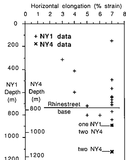
Fig. 12. Greatest elongation, {}^b\varepsilon_1 , vs depth in samples from DOE wells NY No. 1 and NY No. 4. The lowermost data point lies about 100 m above the Salina salt.
