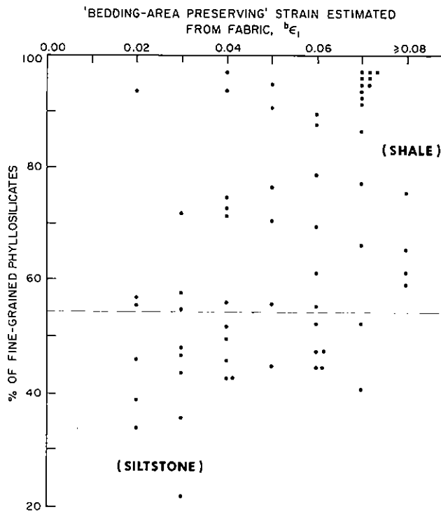
Fig. 11. Greatest elongation, {}^b\varepsilon_1 , inferred from preferred orientation of chlorite basal planes, vs composition (volume-percent of fine-grained phyllosilicates) for the whole data set.
