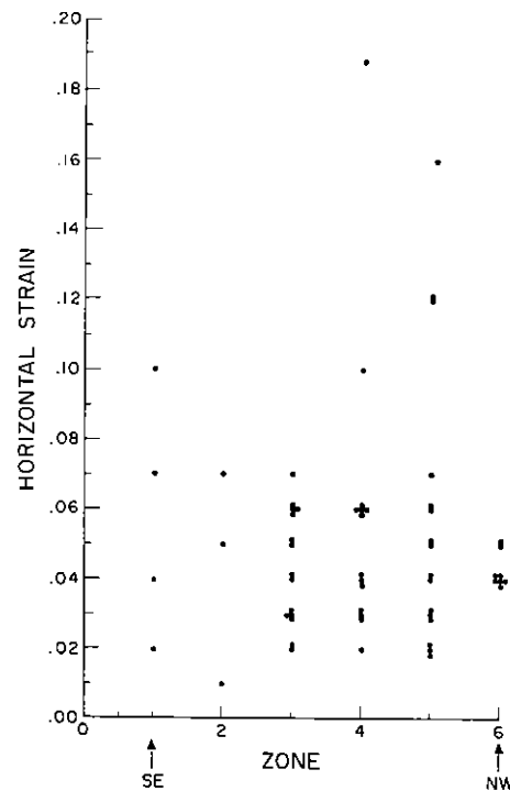
Fig. 5. Horizontal strain, {}^b\varepsilon_1 , vs northwestward distance from the core of the Appalachian fold belt (in six zones).
