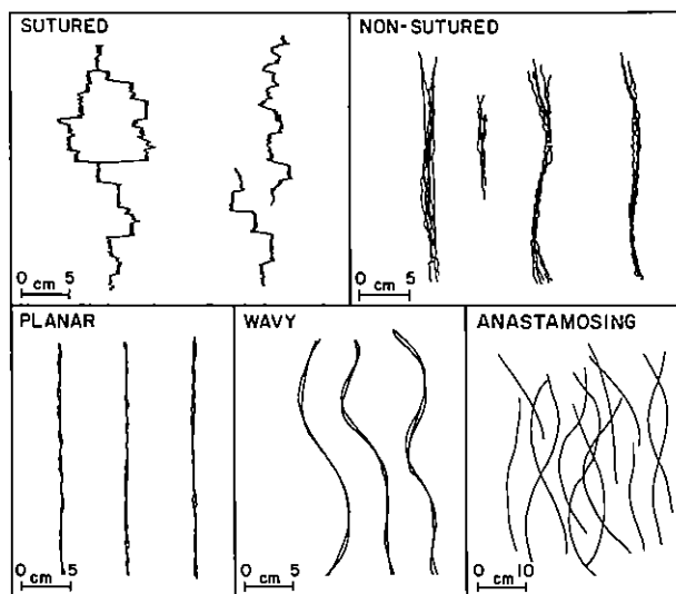
Fig. 2. Patterns of disjunctive cleavage cutting beds.
