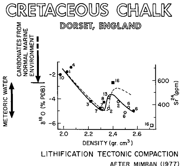
Fig. 7. Relationship between rock density and \delta^{18}\text{O} values for Dorset chalks and calcite veins from exposures of Corfe Castle chalk (square). Dashed line indicates the relationships between density and \text{Sr}^{2+} concentration for Dorset chalk (after Mimran 1977).
